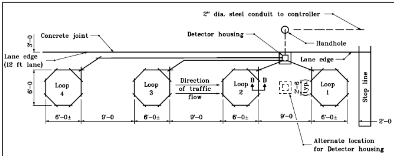
Figure 30. INDOT Typical Traffic Loop Detector Standards for One Lane
