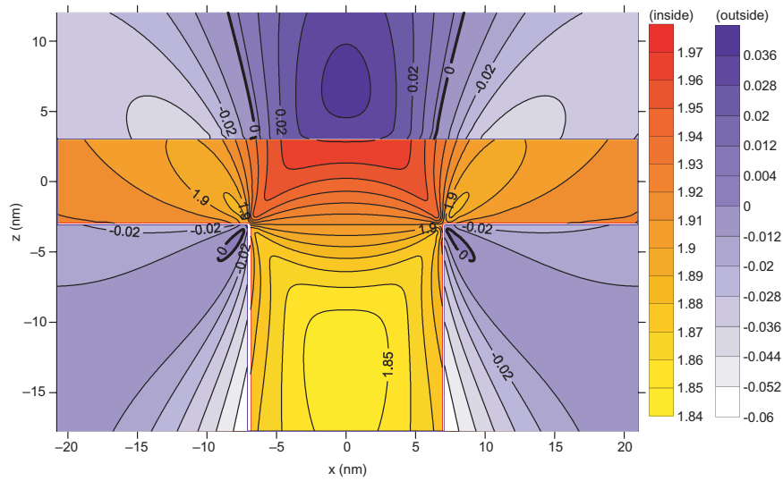
Fig. 3. Hydrostatic strain \gamma_{xx} + \gamma_{zz} distribution inside and outside the T-shaped QWR in the full-plane magnetoelastoelectric substrate.
