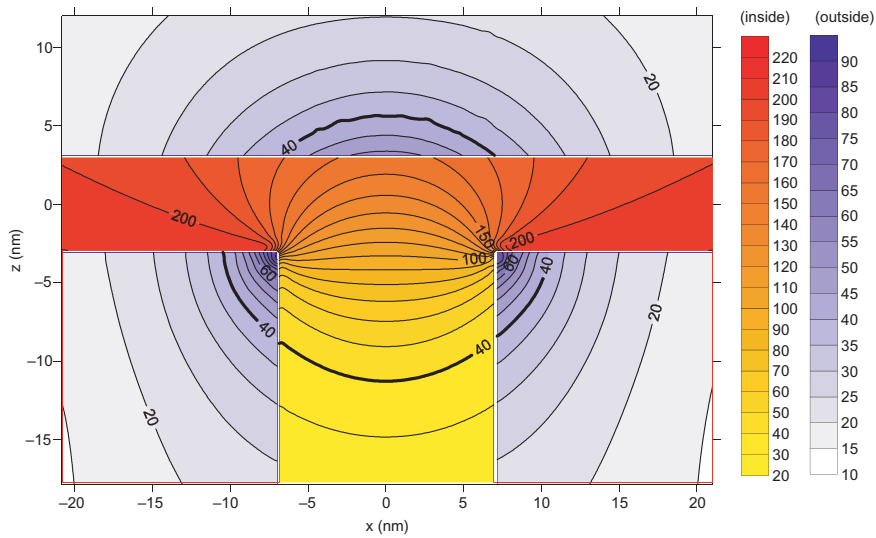
Fig. 4. Total electric field \sqrt{E_x^2 + E_z^2} ( \times 10^7 V/m) distribution inside and outside the T-shaped QWR in the full-plane magnetoelastoelectric substrate.
