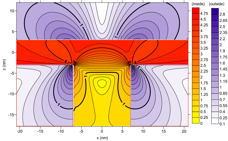
Fig. 5. Total magnetic field \sqrt{H_x^2 + H_z^2} ( \times 10^7 A/m) distribution inside and outside the T-shaped QWR in the full-plane magnetoelastic substrate.
