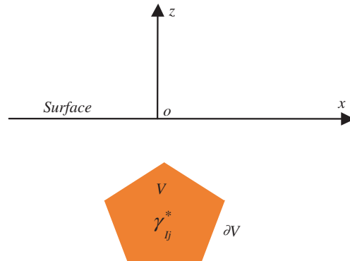
Fig. 1. A general inclusion problem in an anisotropic magneto-electroelastic (x, z) -half-plane ( z < 0 ): an extended eigenstrain \gamma_{IJ}^*(\gamma_{ij}^*, -E_j^*, -H_j^*) within an arbitrarily shaped polygon.
