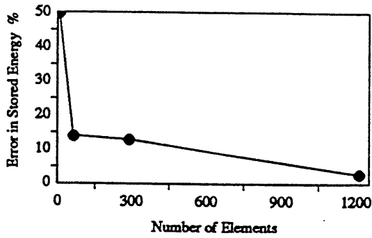
Fig. 7. Error convergence plot.
