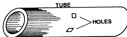
Fig. 4. An Inconel 600 tube with four square through wall holes arranged at 90^\circ . A differential eddy current probe is moved inside to produce an impedance plane trajectory.
